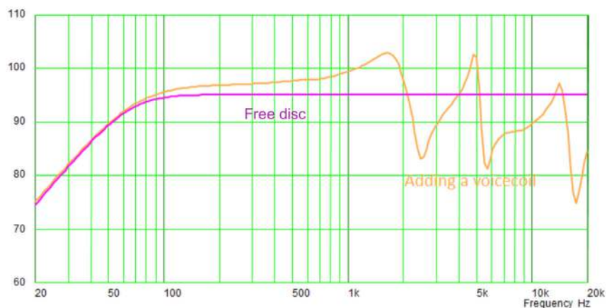
Figure 12. On-axis response of free disc and with voice coil added.
